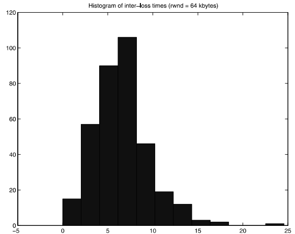
Fig. 12. Case of M = 64 kbytes.
