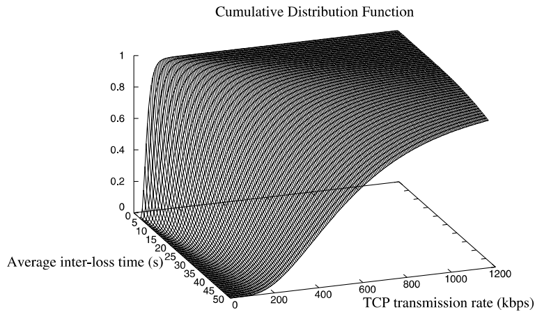
Fig. 5. Unlimited receiver window M = \infty .
