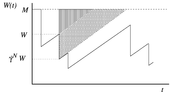
Fig. 1. Area associated with a single loss.
