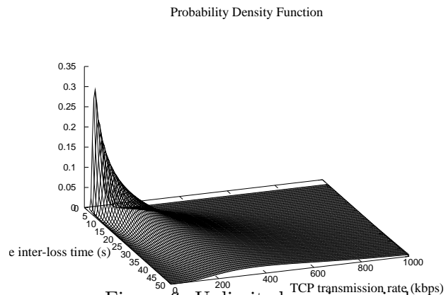
Figure 6: Unlimited receiver window: M = \infty
