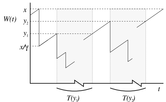
Fig. 2. TCP window.
