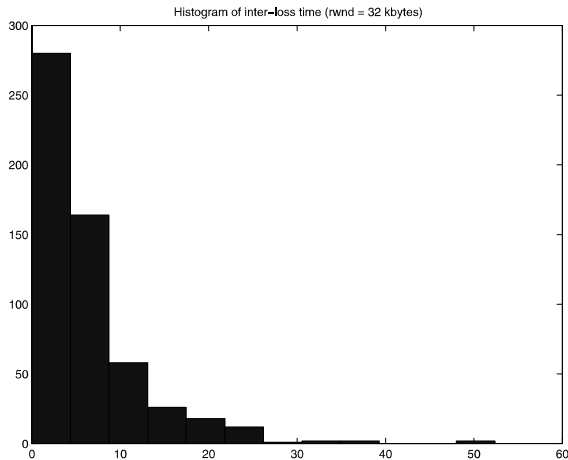
Fig. 10. Case of M = 32 kbytes.
