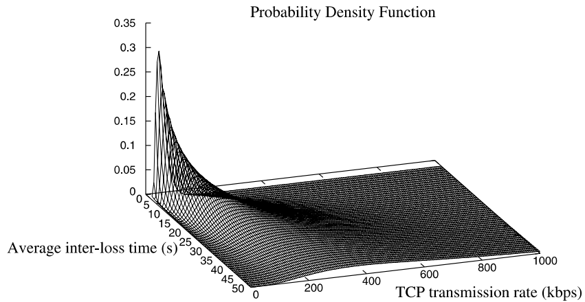
Fig. 6. Unlimited receiver window M = \infty .
