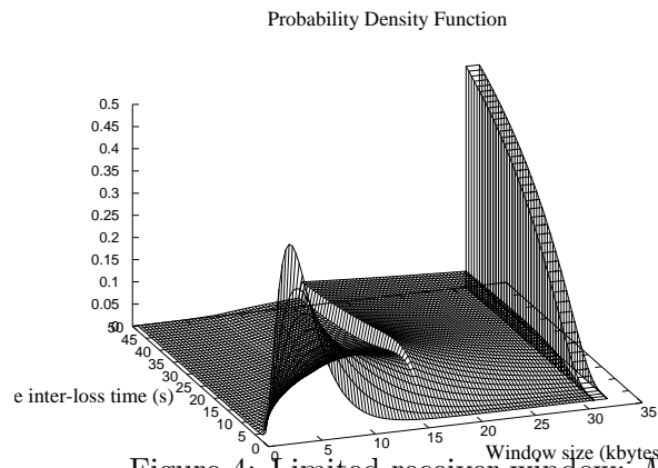
Figure 4: Limited receiver window: M = 32 kbytes
