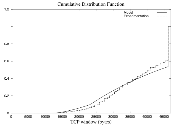
Fig. 8. Receiver window M = 48 kbytes.
