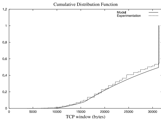
Fig. 7. Receiver window M = 32 kbytes.
