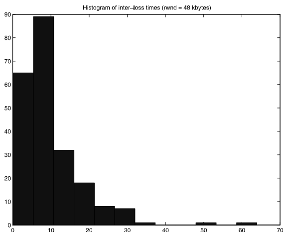
Fig. 11. Case of M = 48 kbytes.
