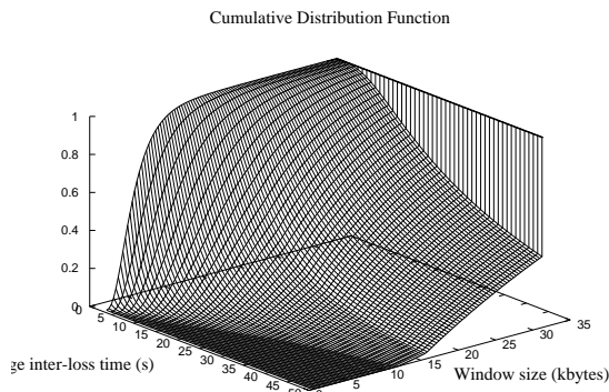
Figure 3: Limited receiver window: M = 32 kbytes
