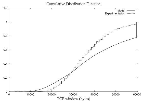
Fig. 9. Receiver window M = 64 kbytes.
