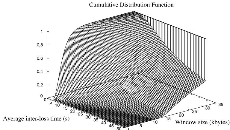
Fig. 3. Limited receiver window M = 32 kbytes.
