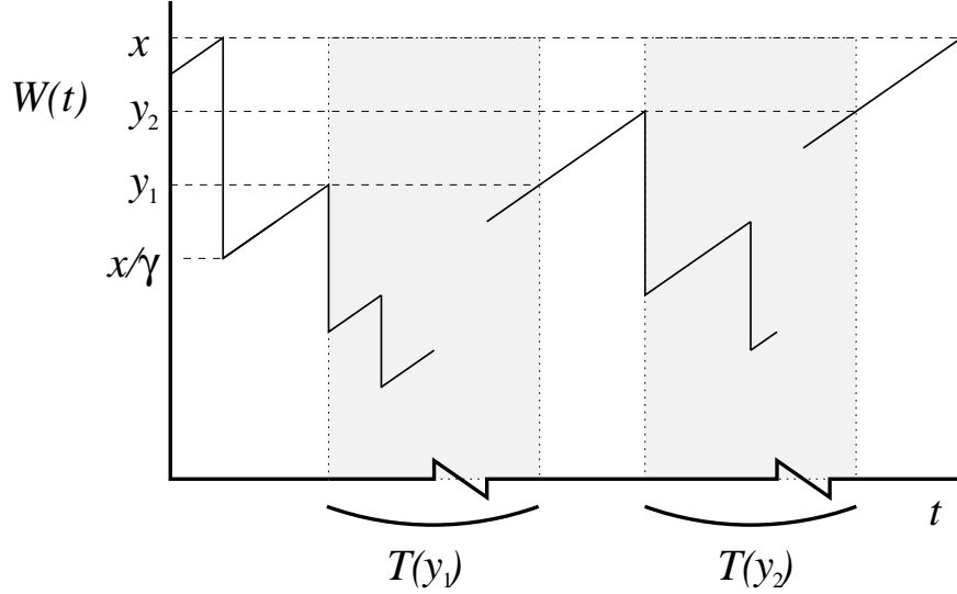
Figure 2: TCP window
