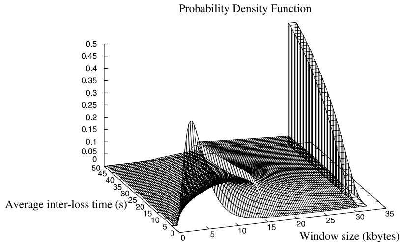
Fig. 4. Limited receiver window M = 32 kbytes.
