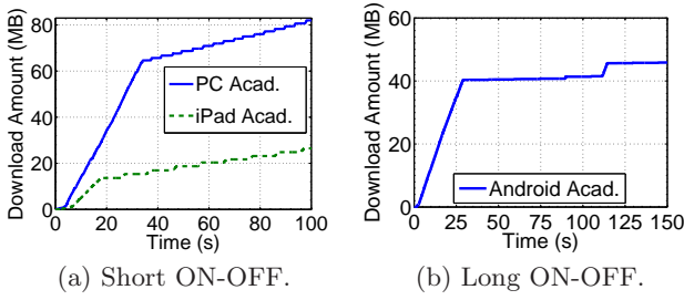
Figure 10: Streaming Strategies used by Netflix. Short ON-OFF cycles for PCs and iPad. Long ON-OFF cycles used for the Android application.
