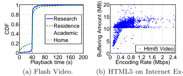
Figure 3: Amount downloaded during the buffering phase. For Flash videos, approximately 40 seconds worth of playback is downloaded in the buffering phase. The buffering amount and the video encoding rate is weakly correlated for HTML5 videos.
