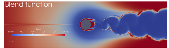
Figure 3. Isocontours of the blending function for the circular cylinder benchmark (Reynolds 10^6 ): for \theta = 1 (in red) the RANS model is activated, wherever 0 < \theta < 1 additional resolved fluctuations are computed, and in the limit \theta \rightarrow 0 (in blue) the LES approach (DVMS in this work) is recovered.
