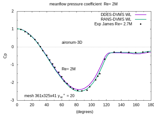
Figure 7. Distribution over the cylinder surface of the mean pressure coefficient. Comparison between experimental data and numerical results at Reynolds 2 \times 10^6 .
