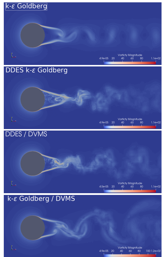
Figure 6. Circular cylinder, Reynolds 10^6 : instantaneous isocontours of the vorticity magnitude. From top to bottom: RANS, DDES, DDES/DVMS and RANS/DVMS.
