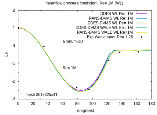
Figure 5. Distribution over the cylinder surface of the mean pressure coefficient. Comparison between experimental data and numerical results at Reynolds 10^6 .
