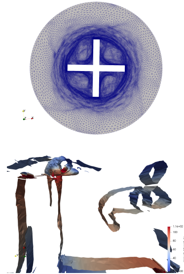
Figure 8. DDES computation of a rotating mixing device with a mesh adaptative Chimera approach (horizontal cut). View of the mesh and of Q-factor (colored with velocity magnitude) after the vertical upper blade.
