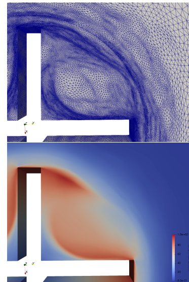
Figure 9. DDES computation of a rotating mixing device with a mesh adaptative Chimera approach (horizontal cut). Partial view of the mesh and velocity magnitude.
