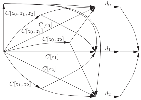
Fig. 8. Modeling the constraints of zones as flows.
