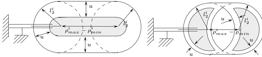
Figure 24: The dextrous workspace for C when only the constraints on link 1 are taken into account (in grey, u = \|\mathbf{CB}_1\| ).
