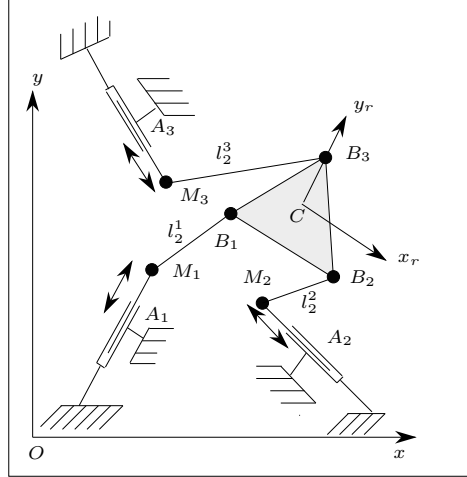
Figure 3: The 3 – PRR planar parallel manipulator
