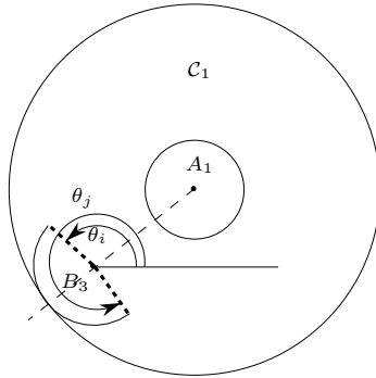
Figure 18: Point B_3 belongs to the boundary of the TOW with the length of link 1 being \rho_{max}^1 . Consequently B_1 lies on a circular arc with center B_3 , radius \|\mathbf{B}_3\mathbf{B}_1\| and angles \theta_i, \theta_j . This arc must be included in the annular region \mathcal{C}_1 and is tangent at some point to the external circle of \mathcal{C}_1 .
