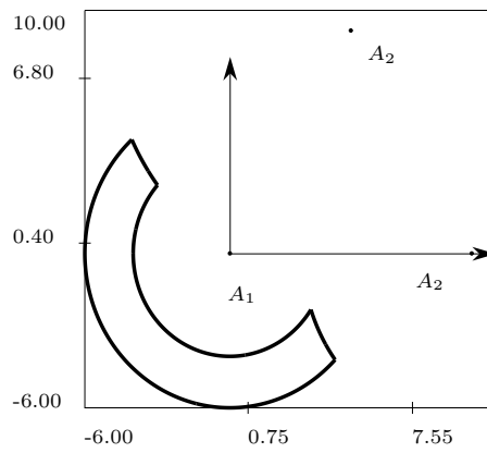
Figure 23: Dextrous workspace for manipulator 4 ( \rho_1 \in [2, 8] , \rho_2 \in [5, 25] , \rho_3 \in [10, 25] , computation time: 80ms).
