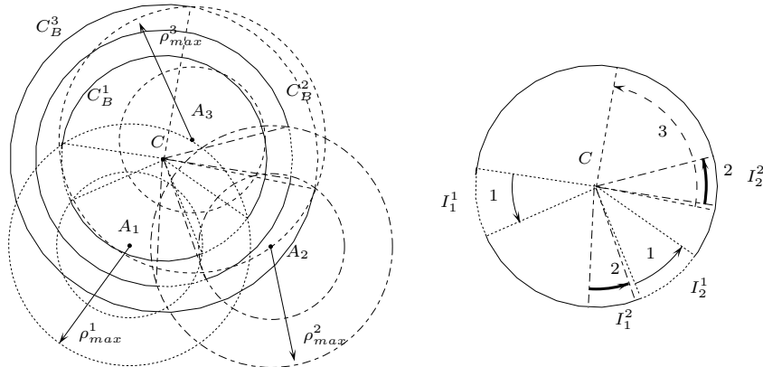
Figure 6: For a given position of C the regions which can be reached by the B_i 's define three lists \{I_l^1\}, \{I_m^2\}, \{I_n^3\} of intervals for the orientation of the moving platform. If C is in the maximal workspace the intersection of these lists must be non empty. On the right it may be seen that the intersection is empty as there is no intersection between \{I_l^1\} and \{I_m^2\} .
