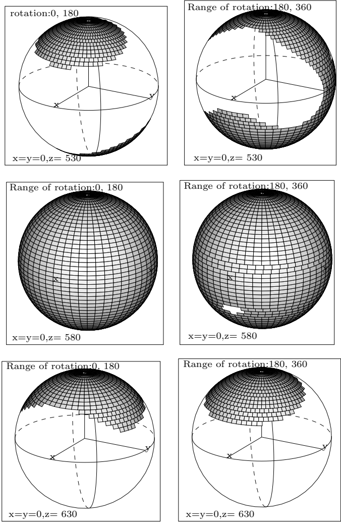
Figure 15: Representation of the possible regions for the extremity of an unit link directed along the z_r axis of the mobile plate when the mobile plate rotates around the z axis after being first rotated around the x axis. The constraints are only the link lengths.
