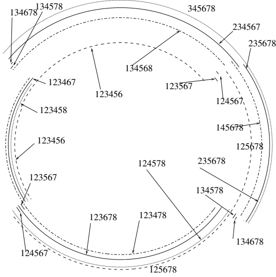
Fig. 2. The possible CC along a circular trajectory. The arcs have the same radius but have been enlarged in order to show the different CC
