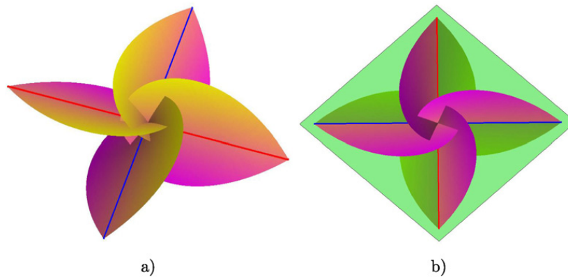
Fig. 3. The minimal surface \overline{r}_1(u, v) and the straight lines on it: (a) \overline{r}_1(u, v) with a_1 = 1 and e_1 = 4 , u, v \in [-4, 4] and the two orthogonal straight lines; (b) another view with plane Z = 0 .
