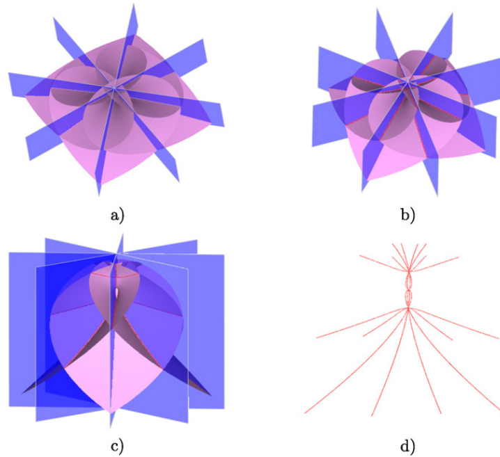
Fig. 2. Symmetric planes and self-intersection curves: (a) \underline{r}_1(u, v) with a_1 = 1 and e_1 = -10 , u, v \in [-4, 4] and its symmetric planes; (b) \underline{r}_1(u, v) with symmetric planes and self-intersection curves (red); (c) another view; (d) self-intersection curves. (For interpretation of the references to color in this figure legend, the reader is referred to the web version of this article.)
