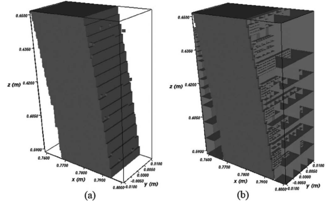
Fig. 2. Workspace definition of a 3-DOF serial anthropomorphic arm, based on joint limits constraints of \pm 30^\circ , evaluated within workspace \mathbf{X} = ([0.76, 0.80], [-0.01, 0.01], [0.59, 0.65])^T . The inner solution of the workspace is shown in (a), while the inner and outer solution (in slightly transparent display) is shown in (b).
