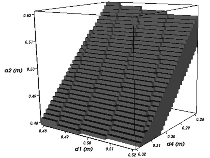
Fig. 3. Design parameters that guarantee that end-effector position \mathbf{X} = ([0.77, 0.78], [-0.01, 0.01], [0.59, 0.60])^T (note: position only) is reachable by the manipulator within the joint limit of 30^\circ .
