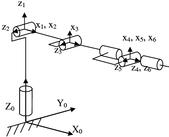
Fig. 1. Frame assignment of the robot used in the discussion.
