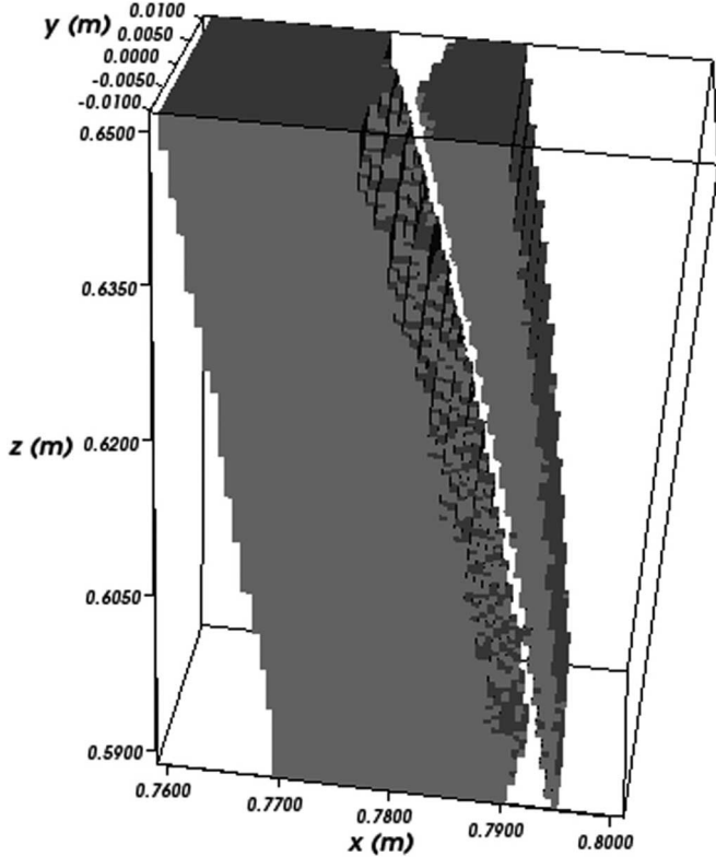
Fig. 4. Constant orientation workspace [as defined in (19)] of the serial manipulator, as defined in Table V, is evaluated as \mathbf{X} = ([0.76, 0.80], [-0.01, 0.01], [0.59, 0.65])^T .
