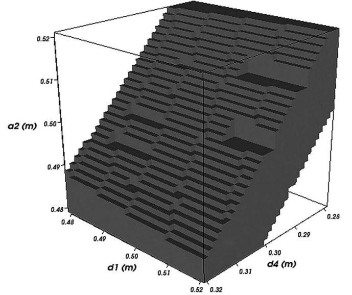
Fig. 5. Design parameters that guarantee constant orientation workspace \mathbf{X} = ([0.773, 0.777], [-0.005, 0.005], [0.598, 0.602])^T is reachable within joint limit constraints of 30^\circ . The constant orientation is defined in (19).
