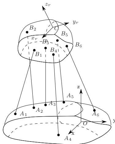
Figure 1: Gough platform
