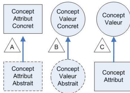
FIG. 4 – Relations interdites
