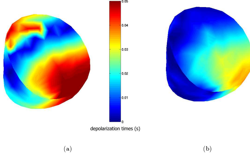
Figure 22: Absolute error on the depolarization times between measures and simulations before (a) and after (b) the global automatic estimation.
