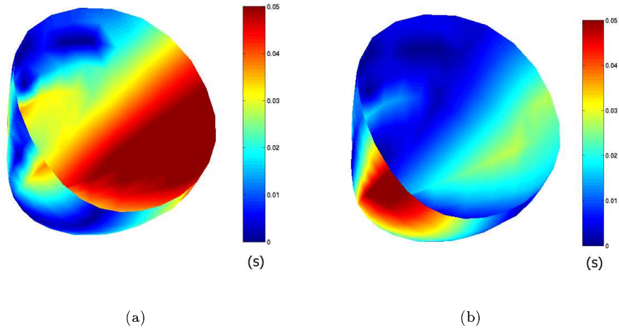
Figure 6: Absolute error on the depolarization times between measures and simulations before (a) and after (b) the global automatic estimation.
