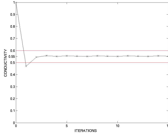
Figure 15: Convergence of the conductivity. Case of non homogeneous conductivity on the region. Expected estimated conductivity: d \approx 0.55 .
