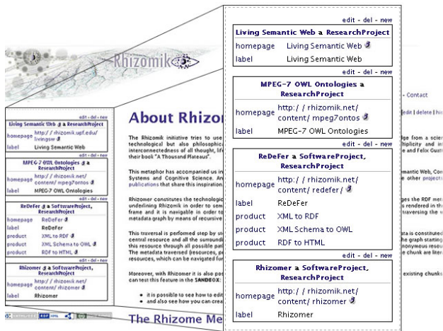
Figure 5. Rhizomik interface with Rhizomer zoom
