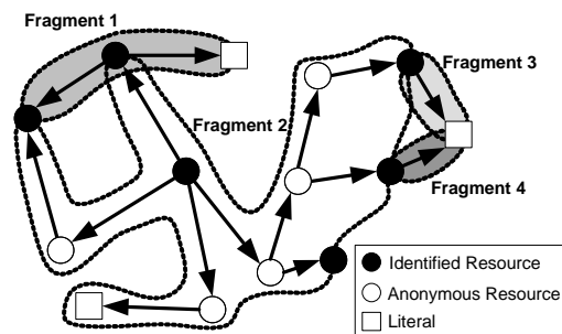
Figure 4. RDF graph and four Rhizomer fragments
