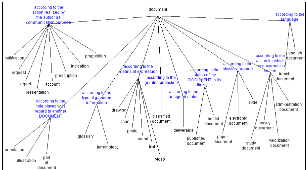
Figure 5 – Different specializations of the notion: document
