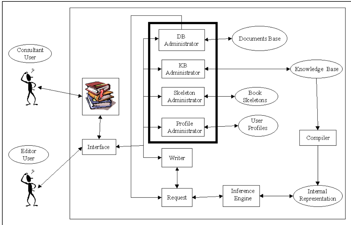
Figure 1 – OM architecture
